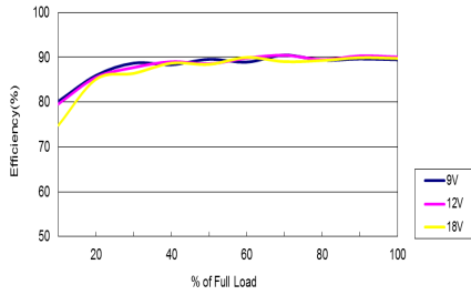
Efficiency Versus Output Current
